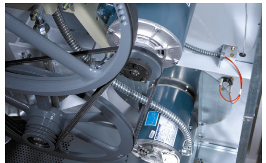
DUAL MOTORS
