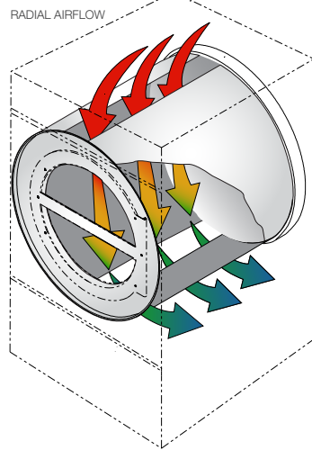
RADIAL AIRFLOW
