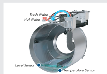
AQUAMIXER™ SYSTEM
